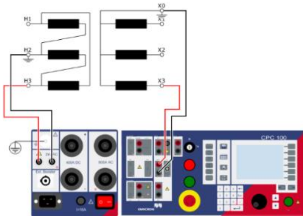
Phase C
