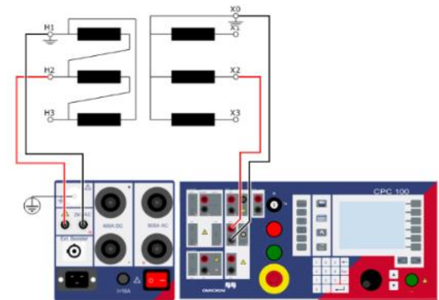
Phase B
