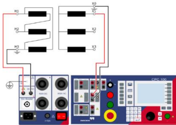
Phase A
