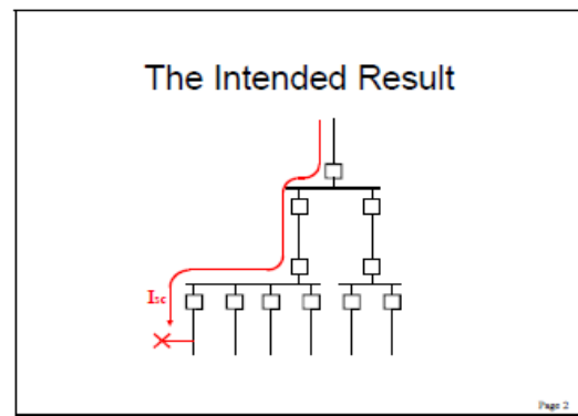
Figure 1 — An example of short circuit flow in a radial system
