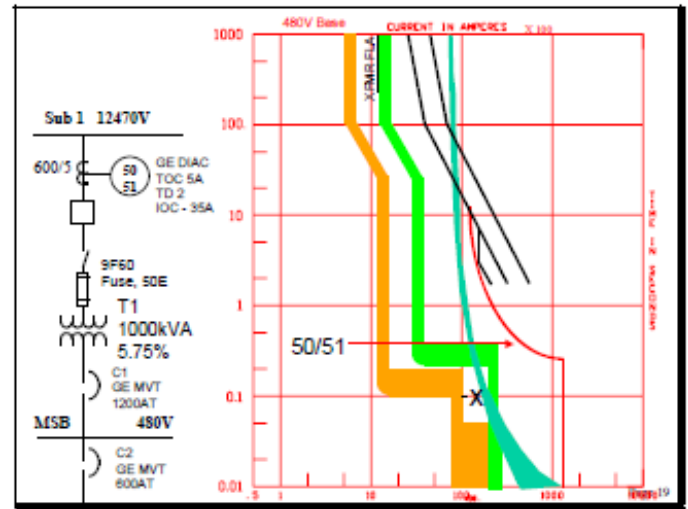
Figure 11 — Unit substation settings
