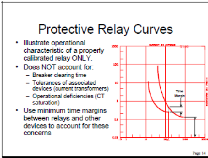
Figure 7 — Protective relay time margins
