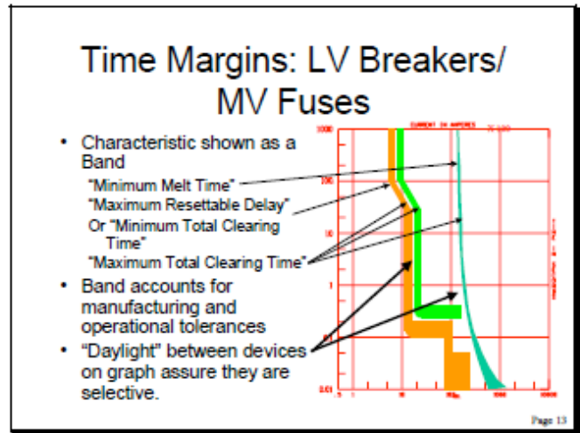
Figure 6 — Overcurrent device curves with minimum and maximum clearing times
