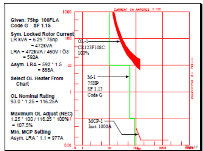
Figure 9 — A motor load and its protection
