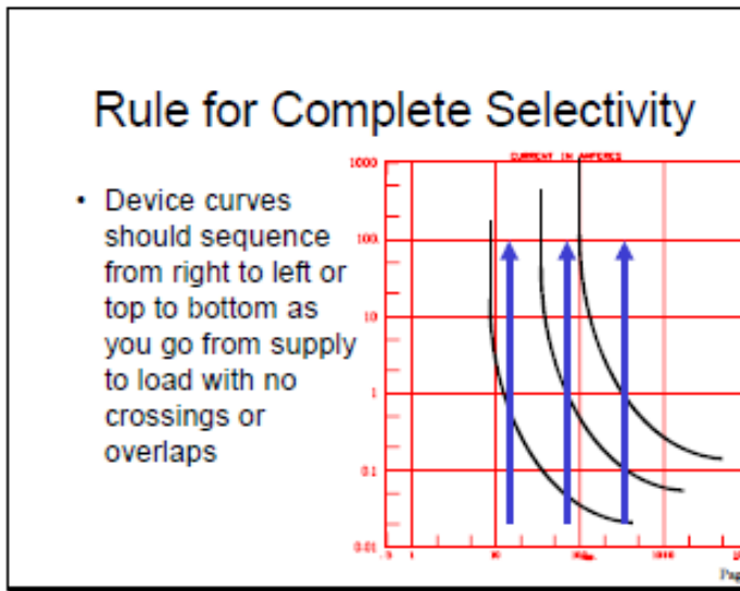
Figure 4 — Identifying complete selectivity
