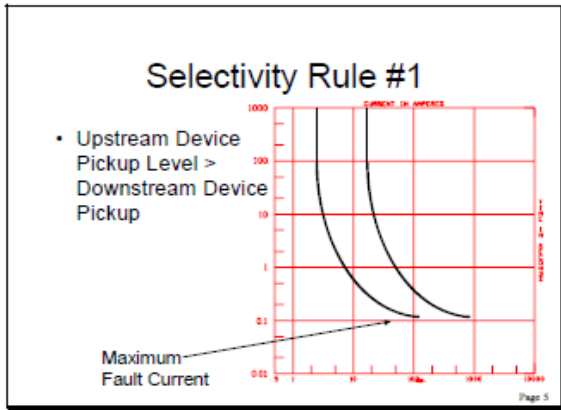
Figure 2 — Creating selectivity by proper selection of pickup settings
