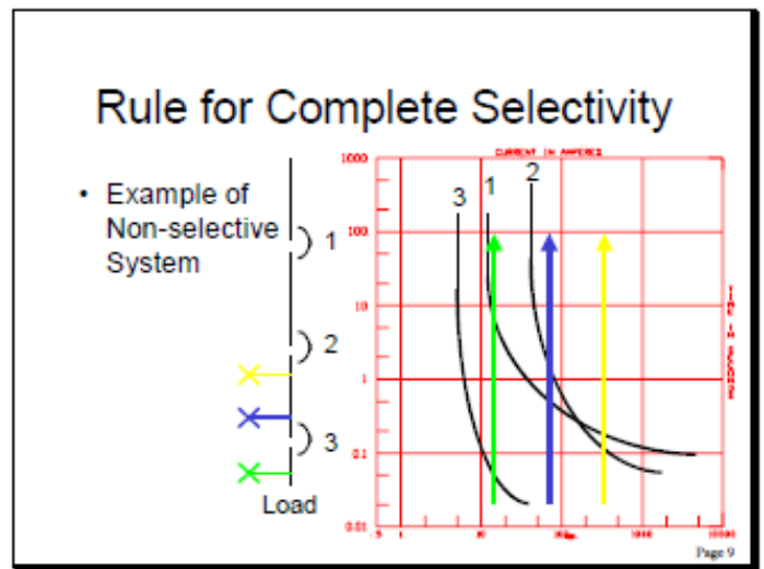
Figure 5 — An example of a non-selective system
