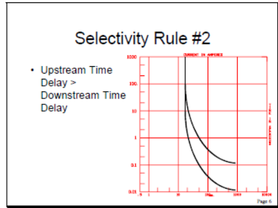
Figure 3 — Creating selectivity by proper selection of delay settings
