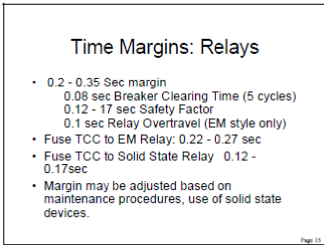
Figure 8 — Recommended relay time margins
