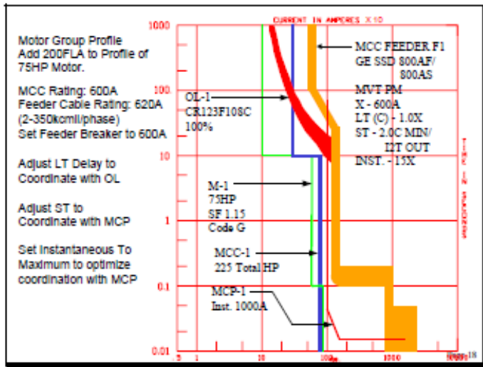
Figure 10 — Adding the feeder breaker supplying the motor control center
